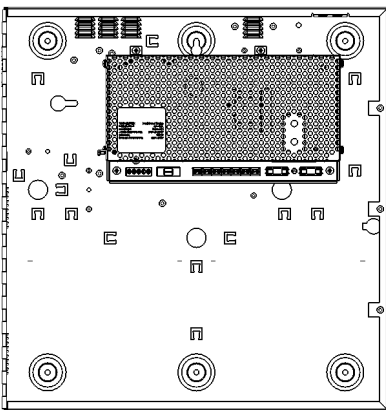
Figure 1 – E Box and Battery mounting
